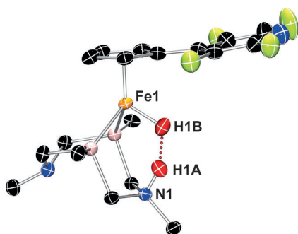
Figure 1. Molecular structure of [\mathbf{1-FeH(NH)}]\text{BARF}_4 determined by neutron diffraction, showing thermal ellipsoids at 50% probability. For clarity, the methyl substituents of the \text{P}^{\text{tBu}}_2\text{N}^{\text{tBu}}_2 ligand, the \text{BARF}_4^- anion, the co-crystallized fluorobenzene molecule, and hydrogen atoms bonded to carbon atoms are omitted. Selected distances (Å) and angles (°) for [\mathbf{1-FeH(NH)}]^+ : H1A...H1B 1.489(10); Fe1–H1B 1.544(7); N1–H1A 1.079(6); H1B–H1A–N1 155.6(8); P1–Fe1–P2 83.62(11).
