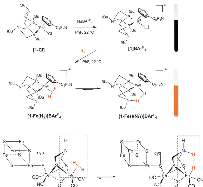
Scheme 1. Top: Synthesis of the 16-electron unsaturated Fe complex (open square indicates a vacant coordination site) and its reaction with \text{H}_2 , leading to the heterolytic cleavage product. Photographs at the right side show NMR tubes containing [\mathbf{1}]^+ and [\mathbf{1-FeH(NH)}]^+ . Bottom: Analogous binding of \text{H}_2 and heterolytic cleavage of \text{H}_2 by the [FeFe] hydrogenase.
